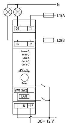
12 V DC power supply – AC circuits switching
