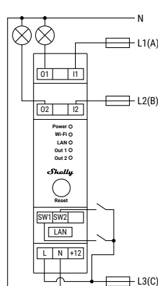
AC power supply – AC circuit switching
