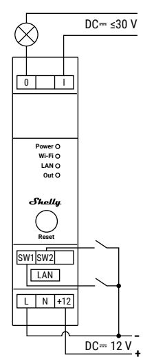
12 V DC power supply – DC circuit switching
