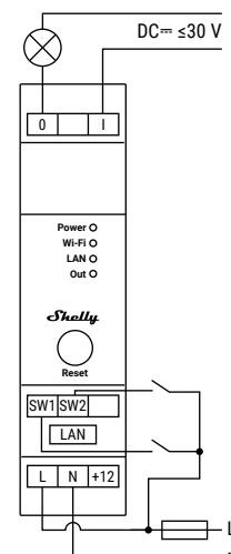
AC power supply – DC circuit switching
