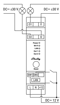
12 V DC power supply – DC circuits switching
