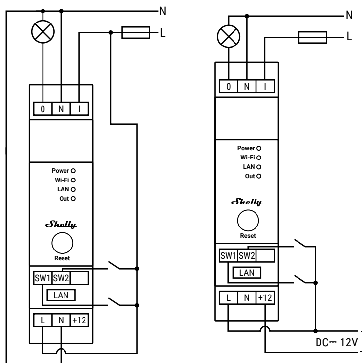
AC power supply – AC circuit switching
