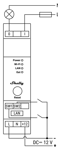
12 V DC power supply – AC circuit switching
