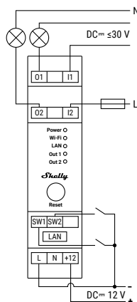
12 V DC – mixed AC & DC circuits switching
