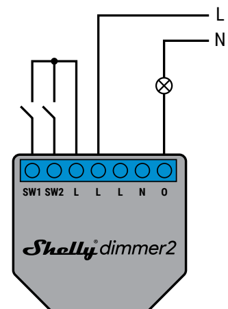
No neutral wiring
