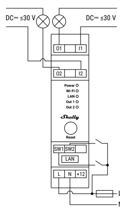
AC power supply – DC circuits switching
