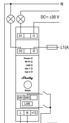
AC power supply – mixed AC & DC circuits switching
