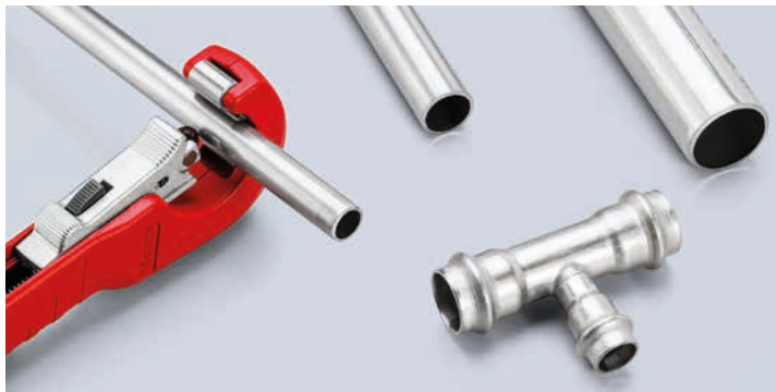
Speed in everyday operation: the QuickLock one-hand locking mechanism enables the cutting wheel to slide onto any pipe diameter with a single press of the thumb
