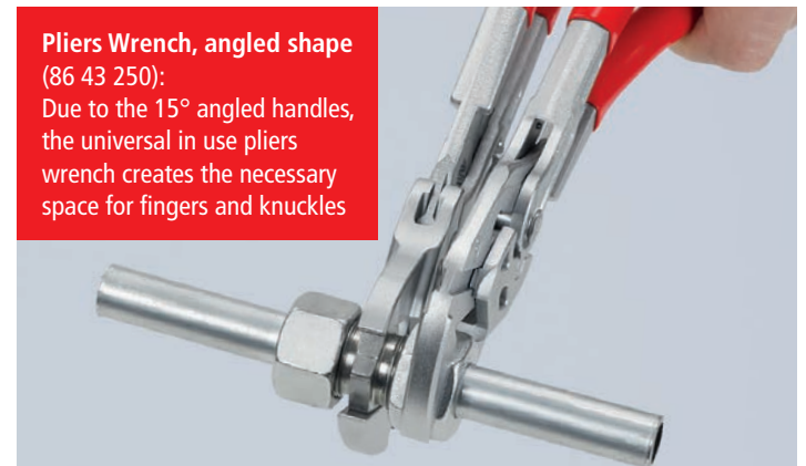
86 43 250 \sphericalangle 15^\circ
