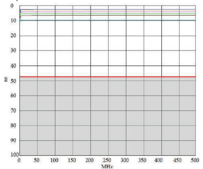
Delay skew
