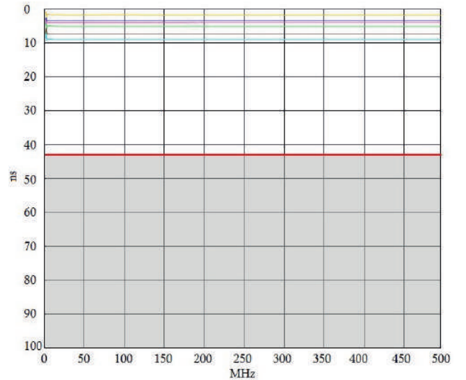
Delay skew
