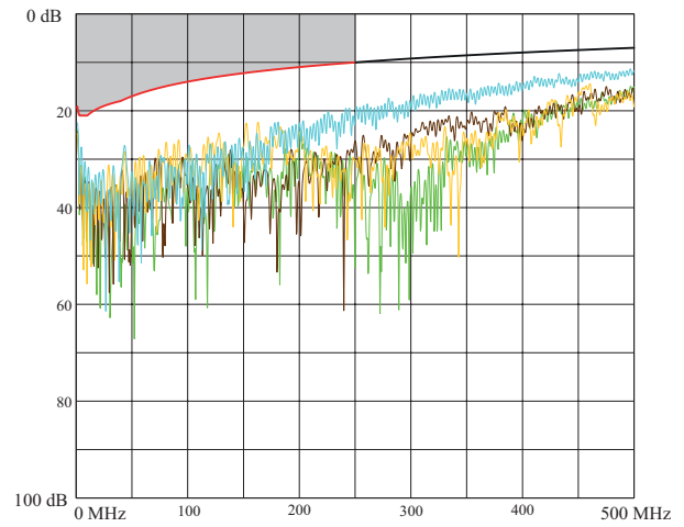
Return loss
