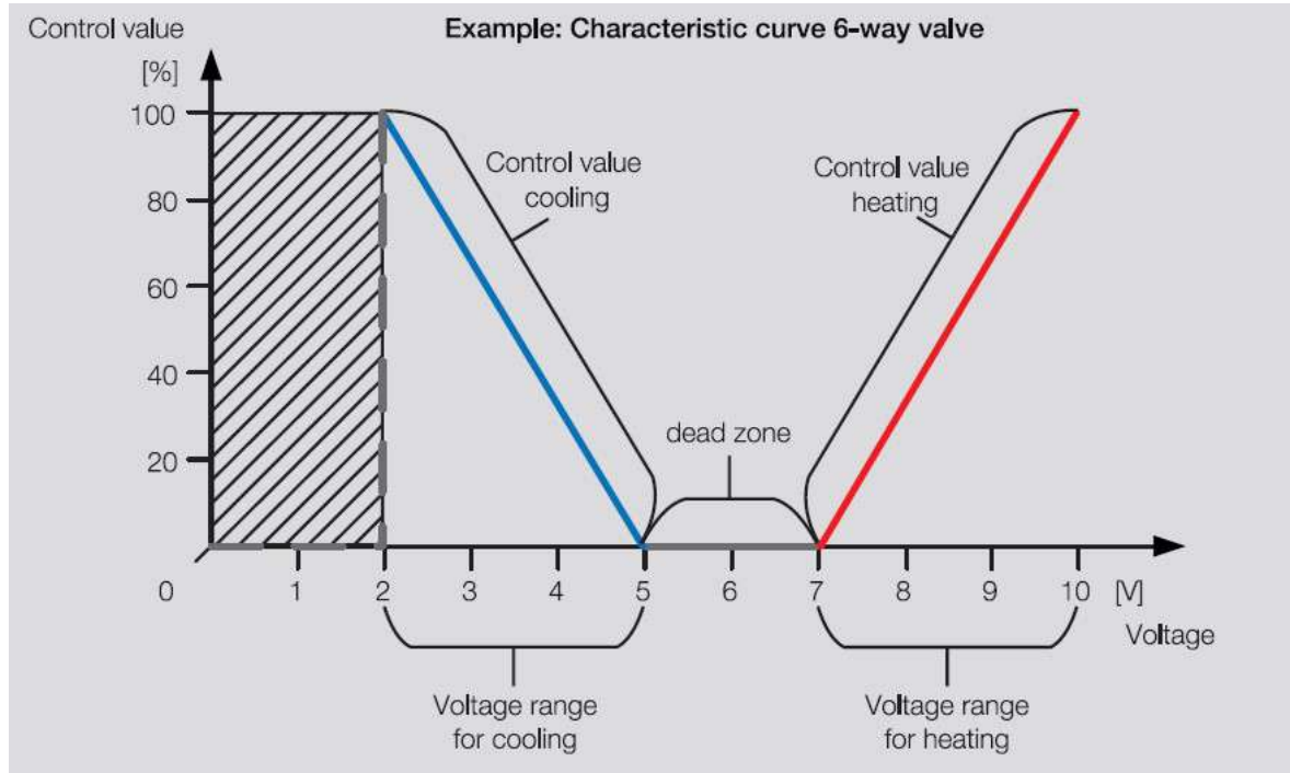
6-way valve
