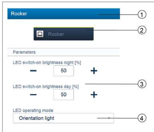
Fig. 52: Rocker settings
