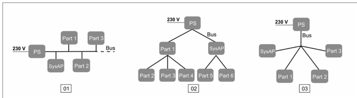
Fig. 3: Possible topologies
