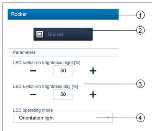
Fig. 56: Rocker settings
