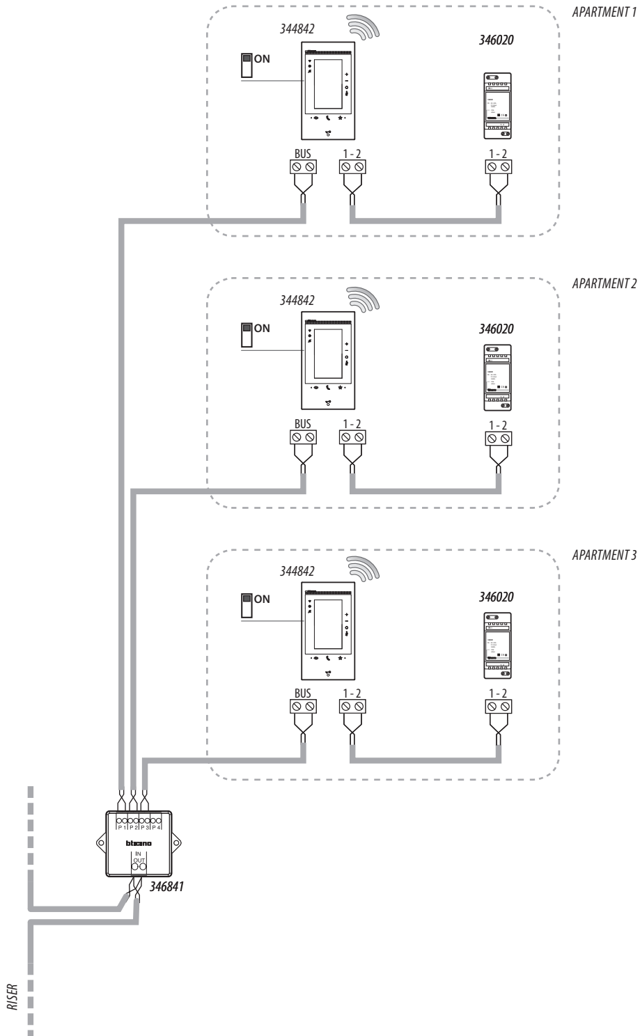
DIAGRAM 1 - EXAMPLE OF MULTI-FAMILY SYSTEM WITH POWER SUPPLY
