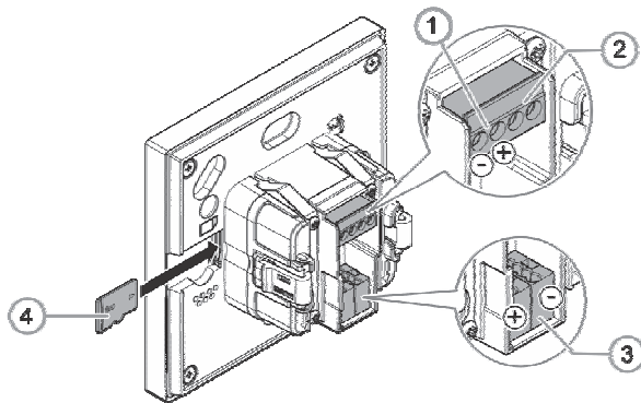
Fig. 4: Device overview of display rear side
