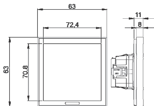
Fig. 7: 4" RoomTouch® RT/U12.86.1-811
