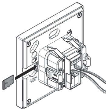
Fig. 37: Inserting the micro SD card (SDHC)
