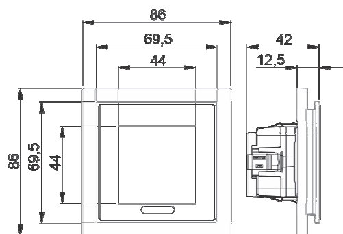
Fig. 8: ABB SmartTouch® 2.4" SD/U12.70.1-4015
